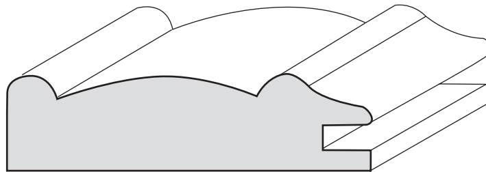
CABINET DOOR RAIL CDR-01 3/4" x 3"
