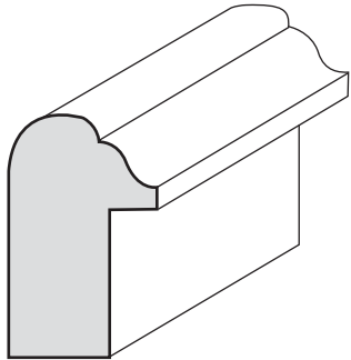
BACK BAND BB-01 3/4" x 1 1/4" Also Available in: BB-02 3/4" x 1 1/8"
