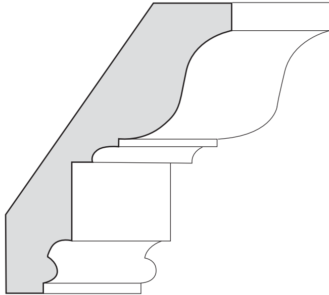
CABINET CROWN CC-01 3/4" x 4 1/8"
