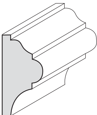
COLONIAL PM-17 3/4" x 1 1/2"
