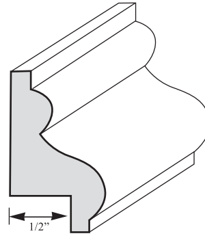
PM-02 3/4" x 1 3/8" Also Available in: PM-03 5/8" Rabitt
