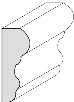
COLONIAL PM-09 5/8" x 1 5/8"
