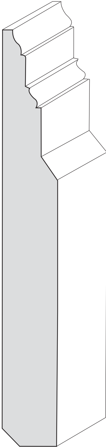
TODUR B-30 1" x 8 1/4"
