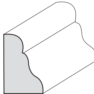
QUARTER ROUND QR-08 3/4" x 1 1/8"
